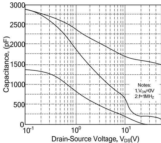
Capacitance Characteristics
